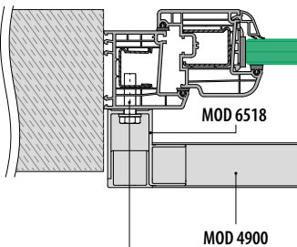
Rammemontering
