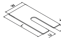
Shims, sidemontert
